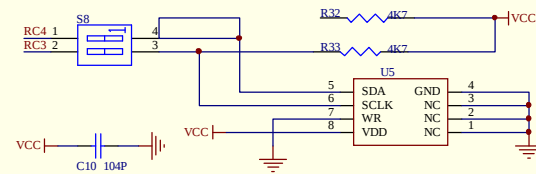
24CX I2C EEPROM
