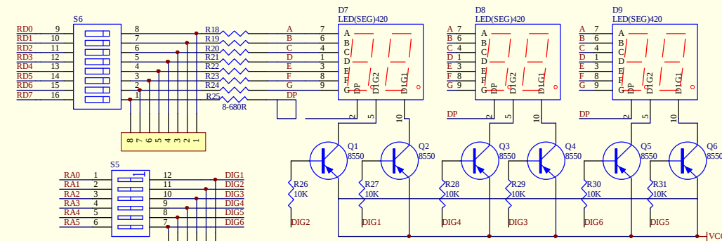
7-SEGMENT DISPLAY
