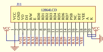
12864LCD
