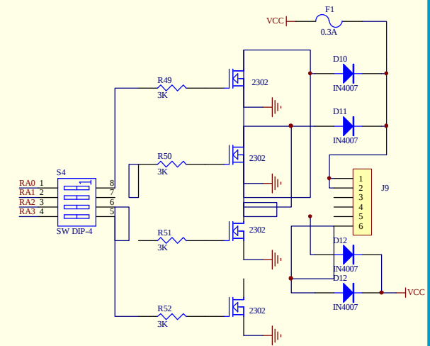
STEPPER MOTOR
