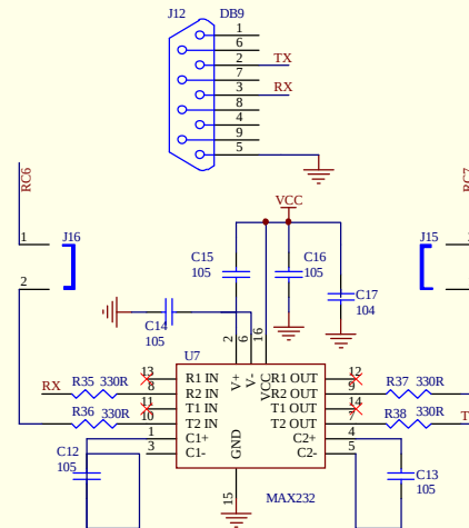
RS232 COMMUNICATION
