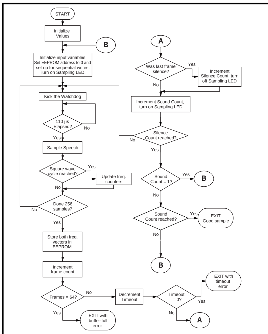
Figure 4 —Every 110 \mu s, the square-wave input is sampled and several options are considered, depending on the state of the frame, zero-crossing, silence, and sound counts. The state machine effectively captures the input utterance, while rejecting short bursts and input errors due to excessive background noise.
