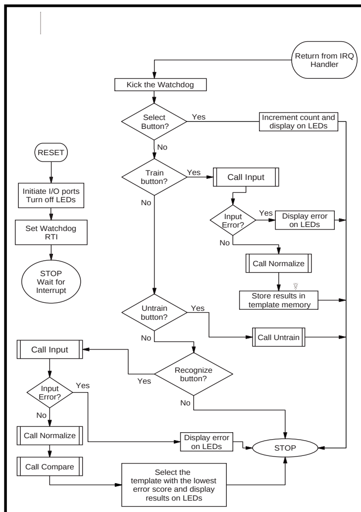
Figure 3 —The main routine performs the event handler. Events are generated by an interrupt caused by pressing a push button or by system reset. The events dispatched are Select, Train, Untrain, and Recognize.
