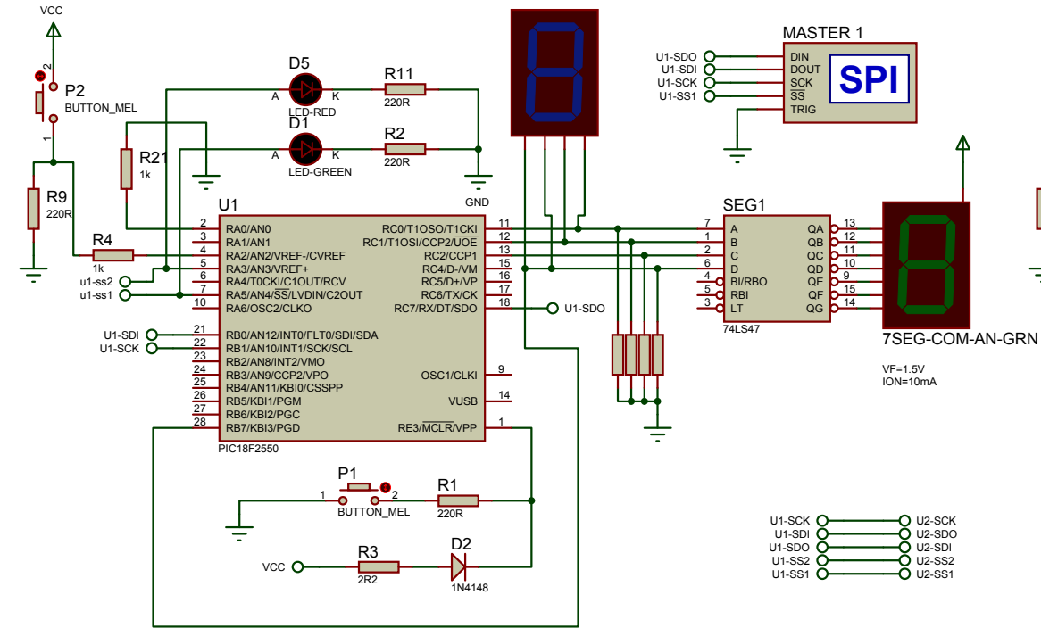
7SEG-BCD-BLUE
