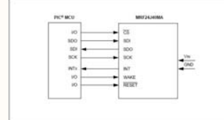
FIGURE 2-2: MICROCONTROLLER TO MIF24A800A INTERFACE
