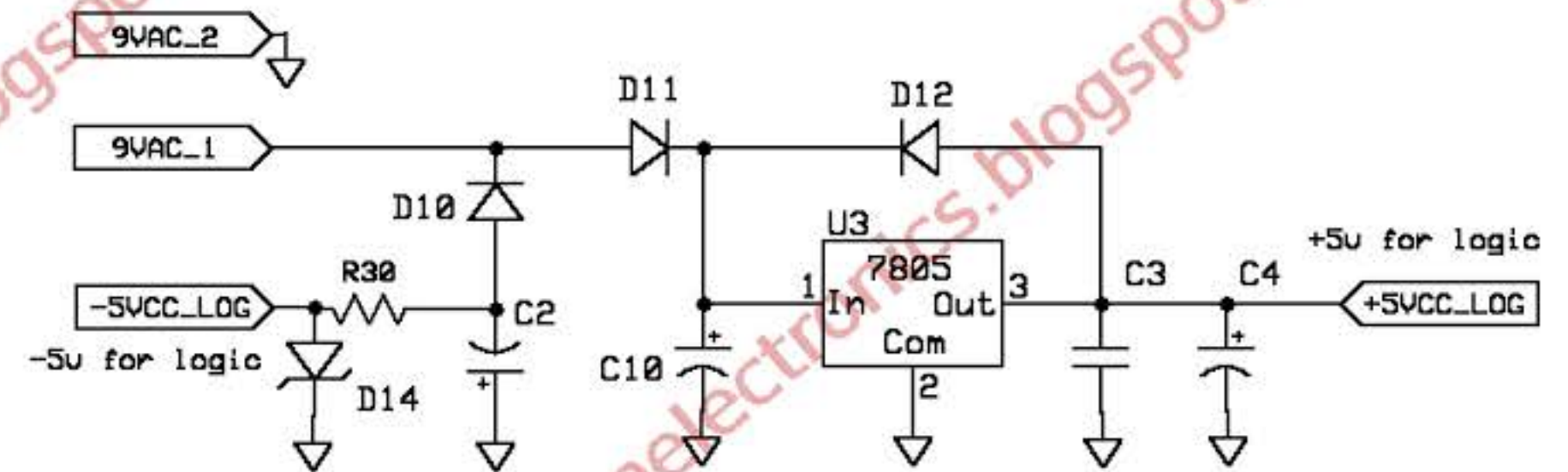
Power regulation
