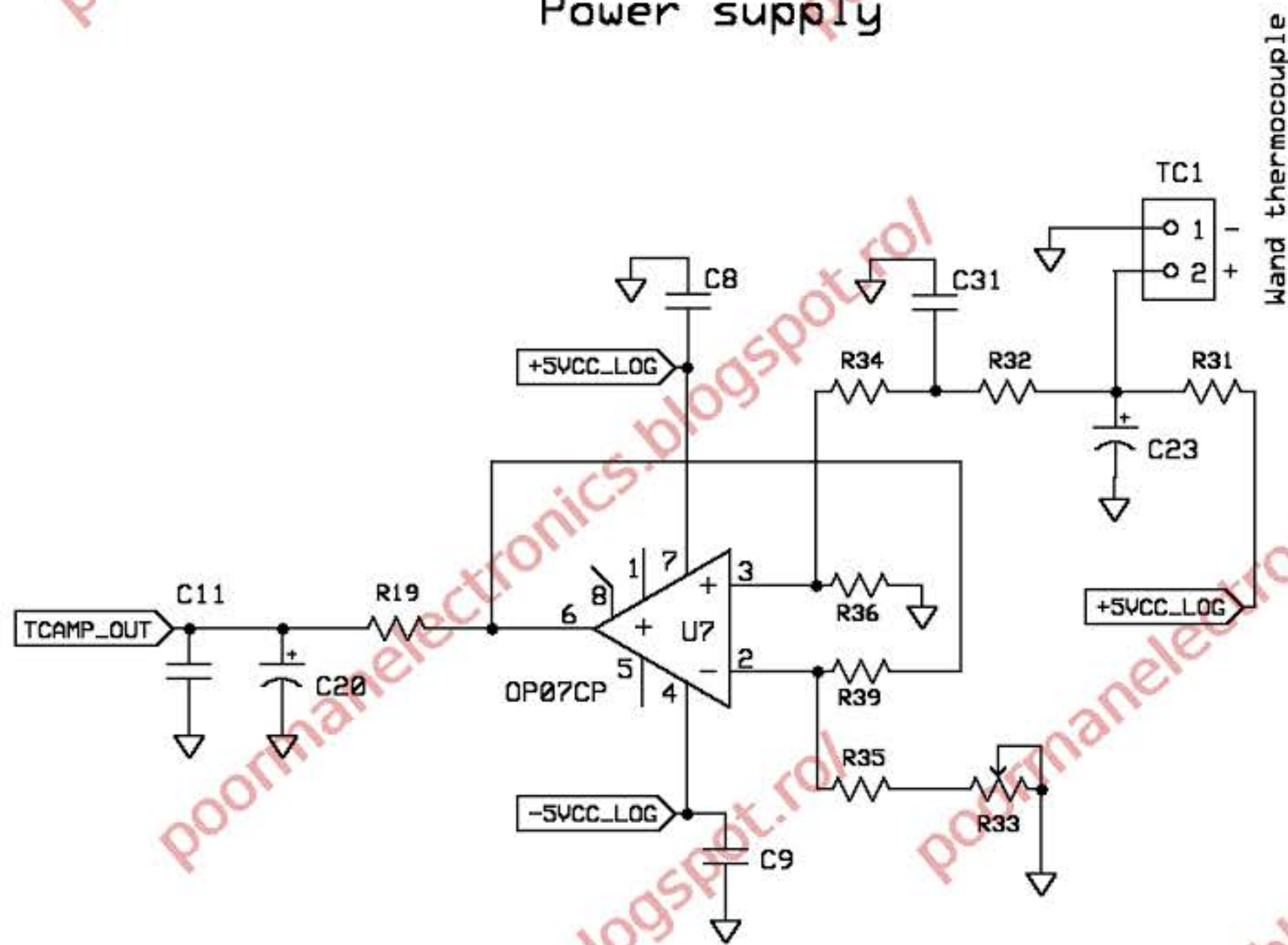
Thermocouple amplifier
