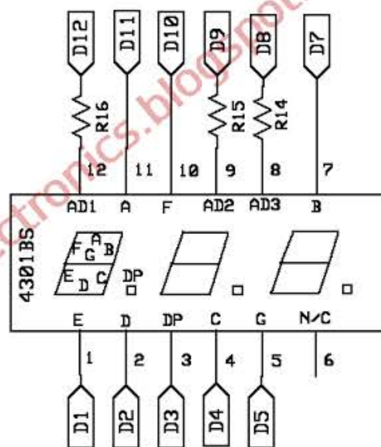
LED display
