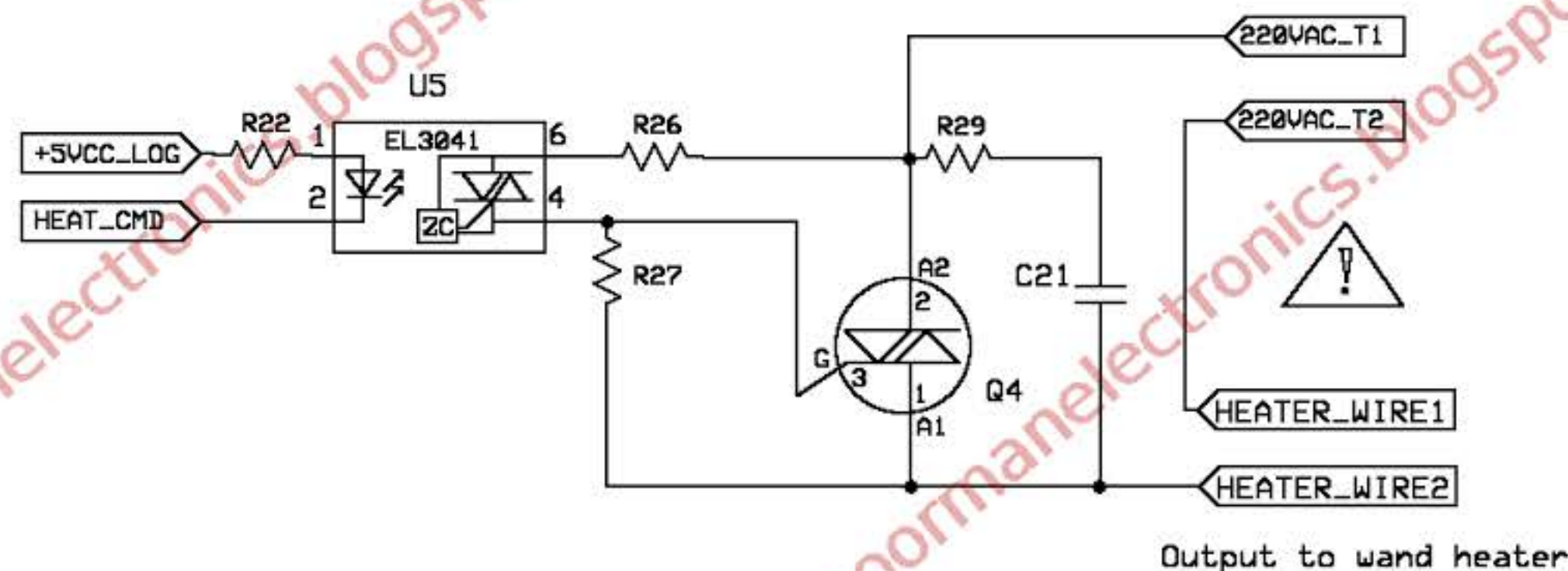
High voltage heater driver
